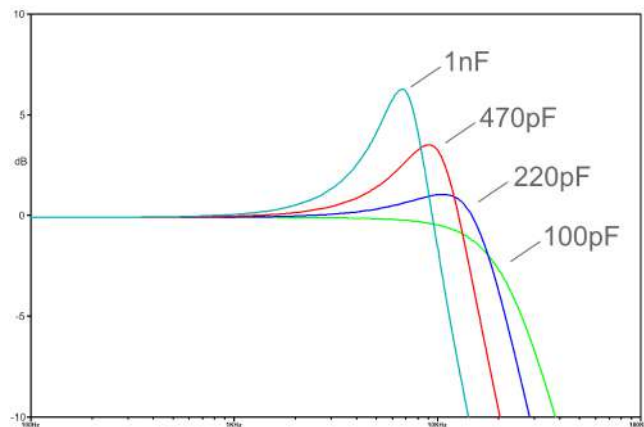
Typical MM cartridge capacitive loading influence on frequency response (with 47 k \Omega resistive load in parallel).
