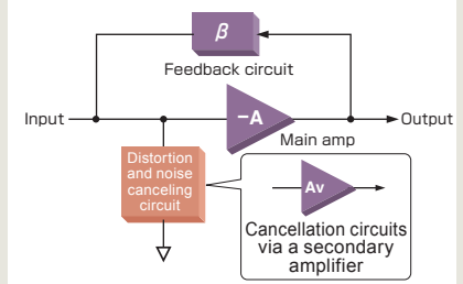
Block diagram of ANCC
